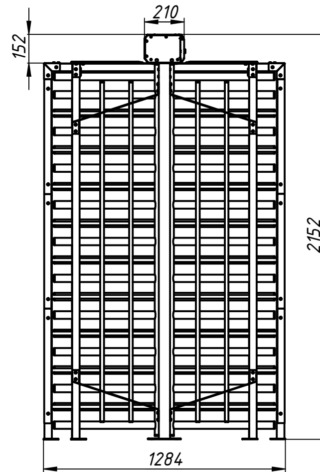
Instalation tamplate
