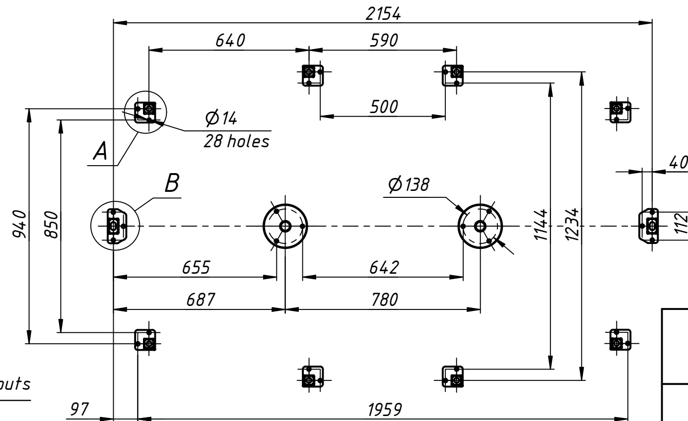
Instalation tamplate
